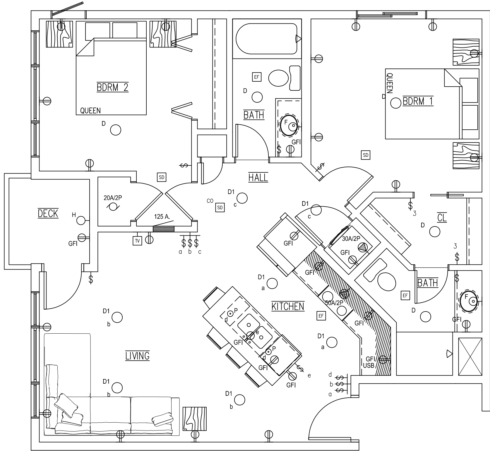
1 UNIT E TYPICAL ELECTRICAL PLAN SCALE: 1/4" = 1'-0"
