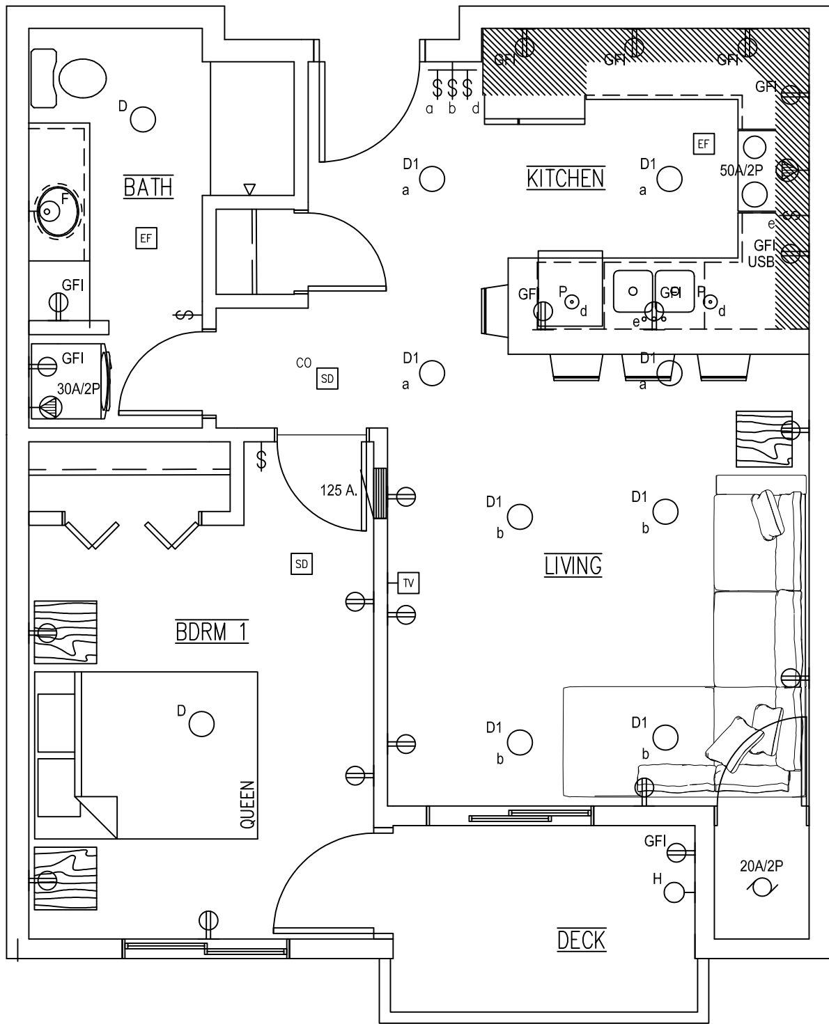
3 UNIT G TYPICAL ELECTRICAL PLAN SCALE: 1/4" = 1'-0"
