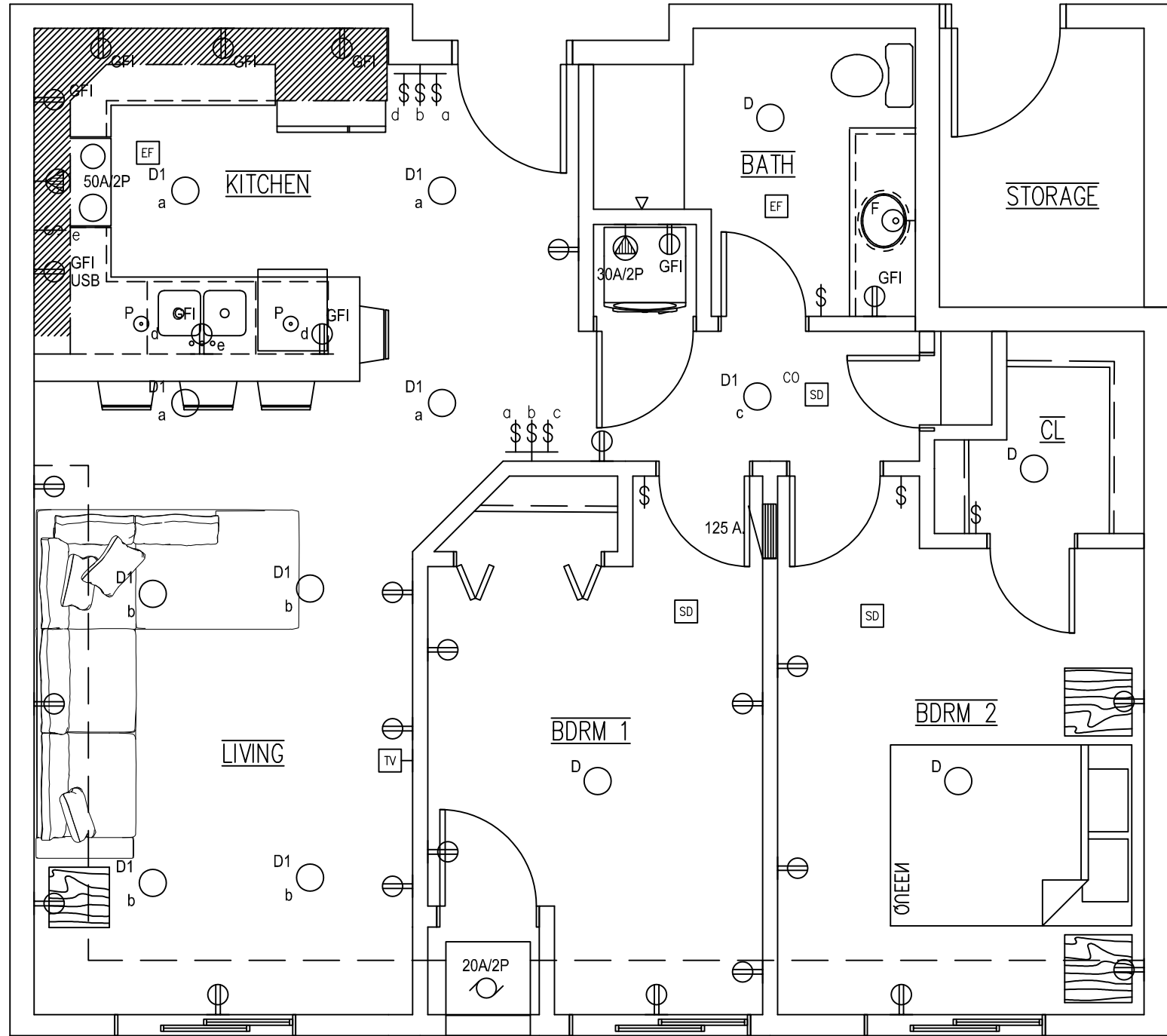
2 UNIT B TYPICAL ELECTRICAL PLAN SCALE: 1/4" = 1'-0"
