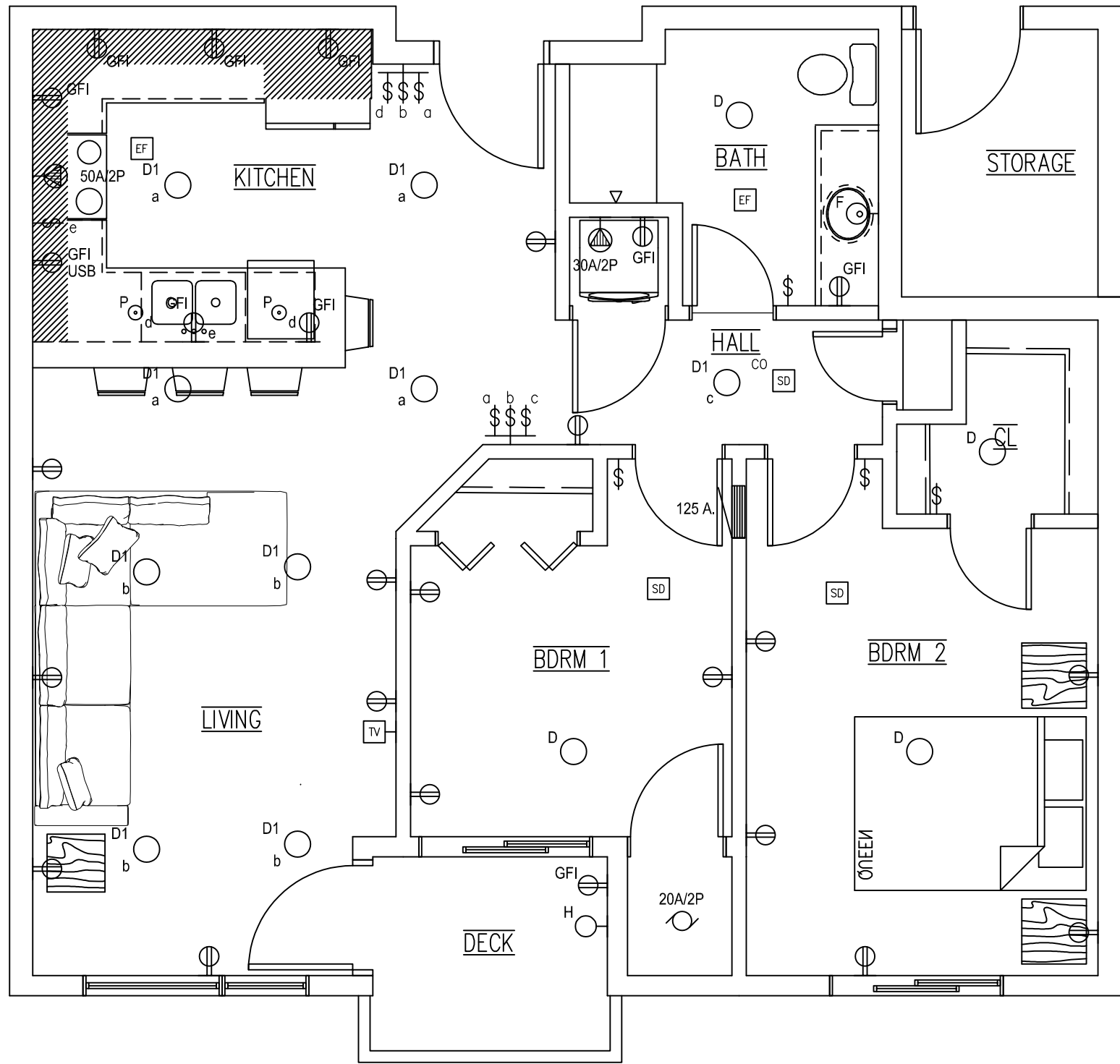
2 UNIT F TYPICAL ELECTRICAL PLAN SCALE: 1/4" = 1'-0"
