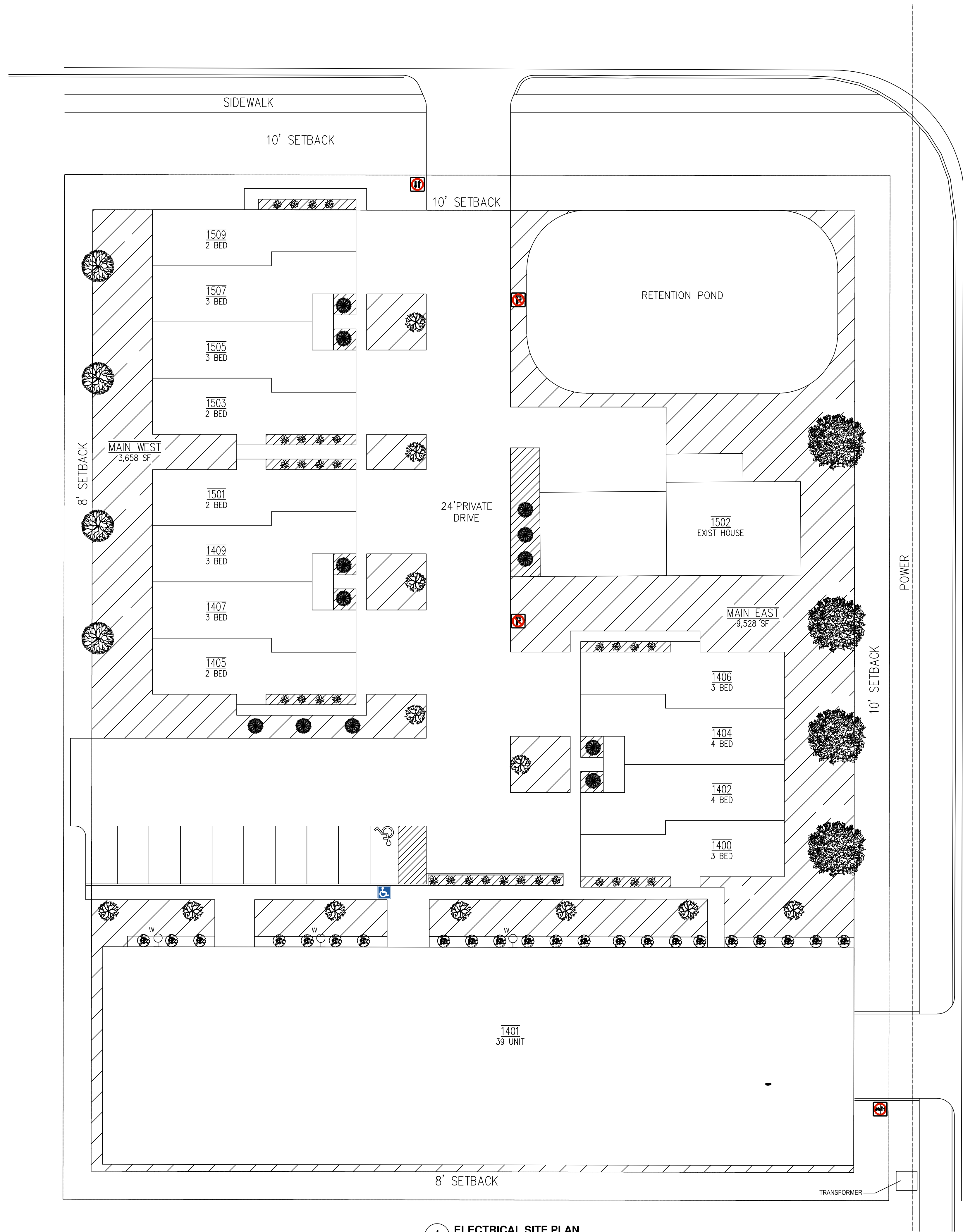
1 ELECTRICAL SITE PLAN SCALE: 1/16" = 1'-0"
