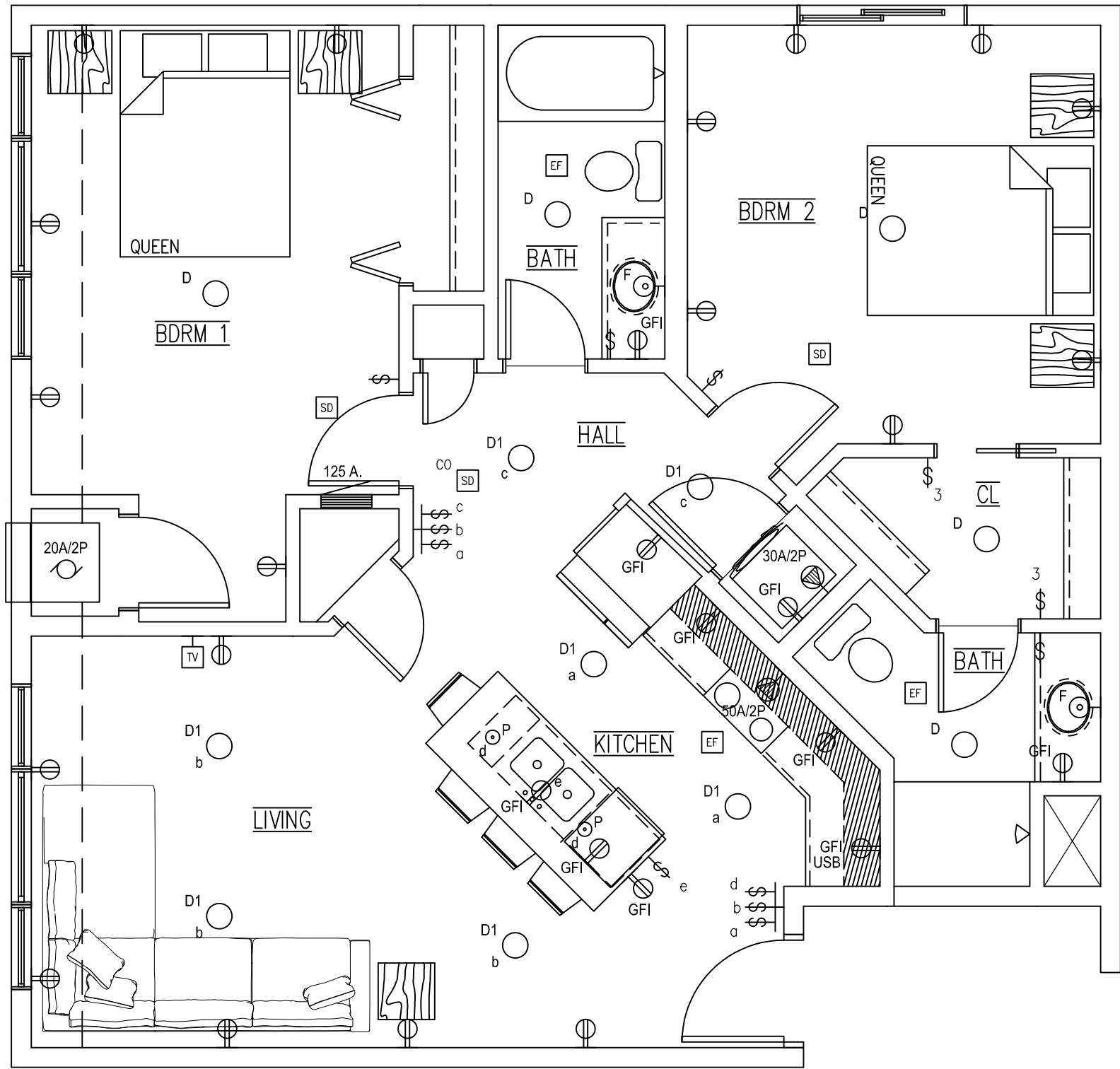
1 UNIT A TYPICAL ELECTRICAL PLAN SCALE: 1/4" = 1'-0"
