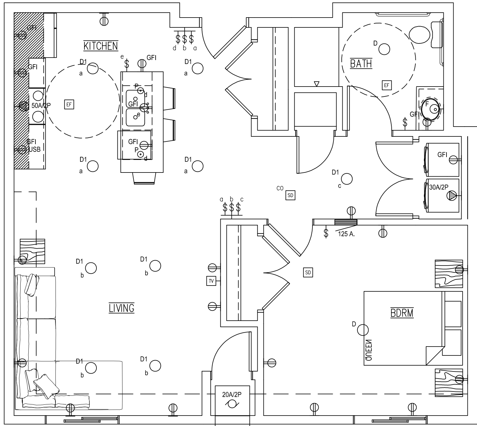
4 UNIT D TYPICAL ELECTRICAL PLAN SCALE: 1/4" = 1'-0"
