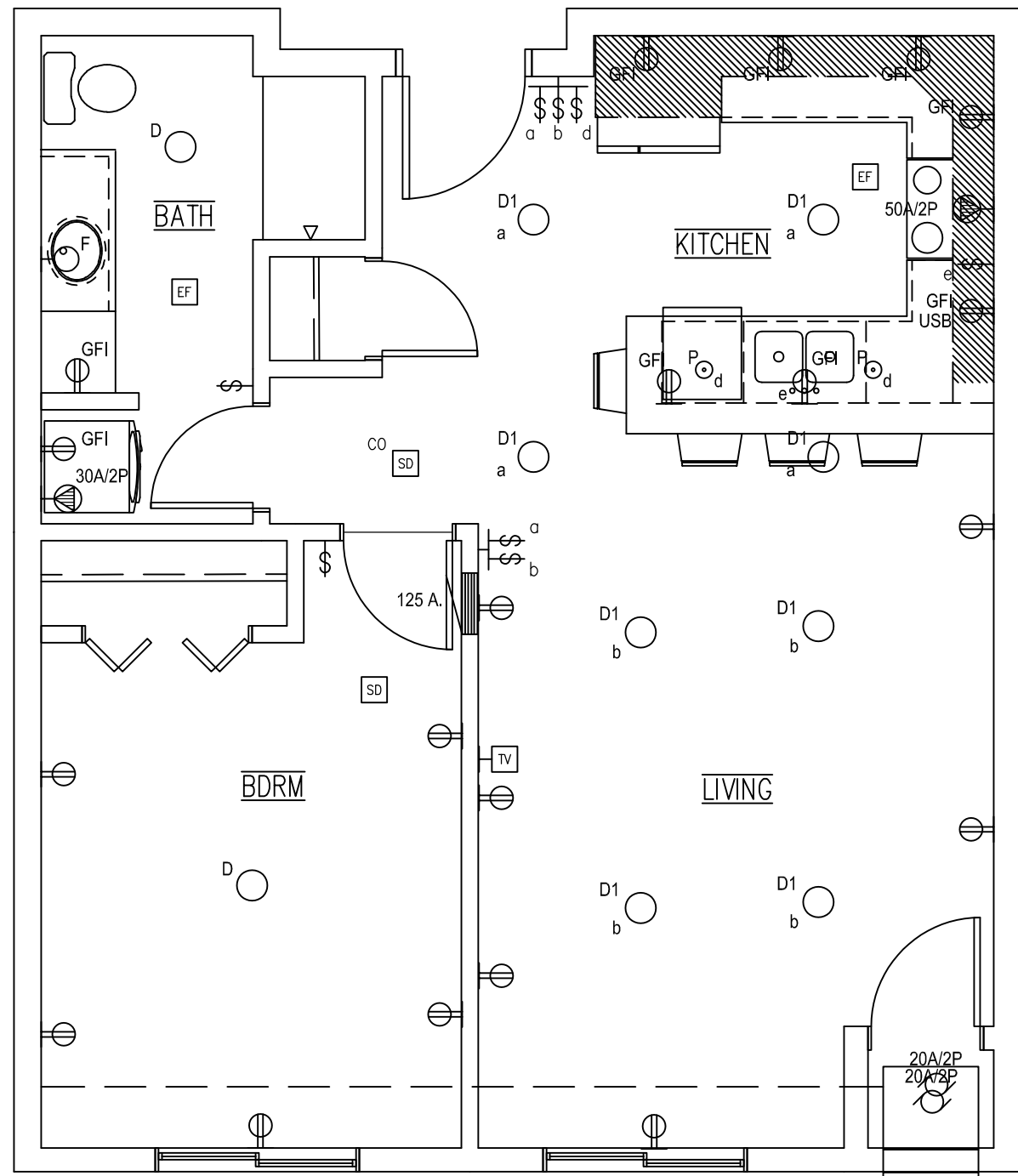
3 UNIT C TYPICAL ELECTRICAL PLAN SCALE: 1/4" = 1'-0"
